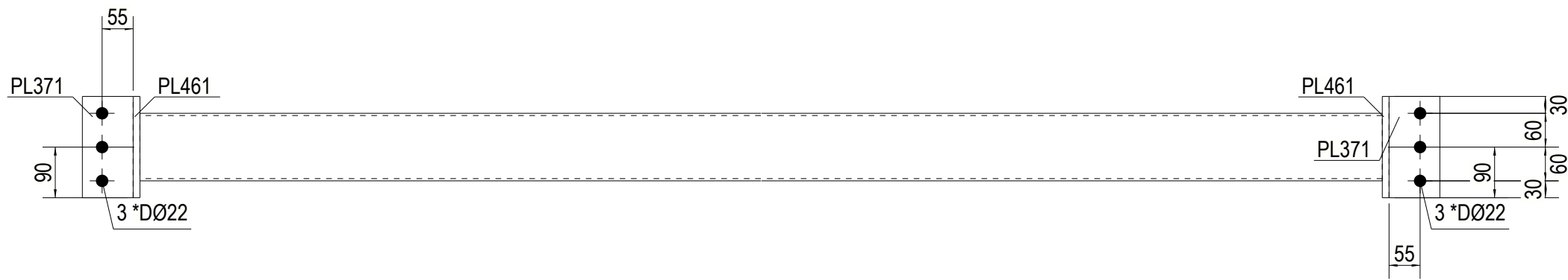
TOP VIEW
