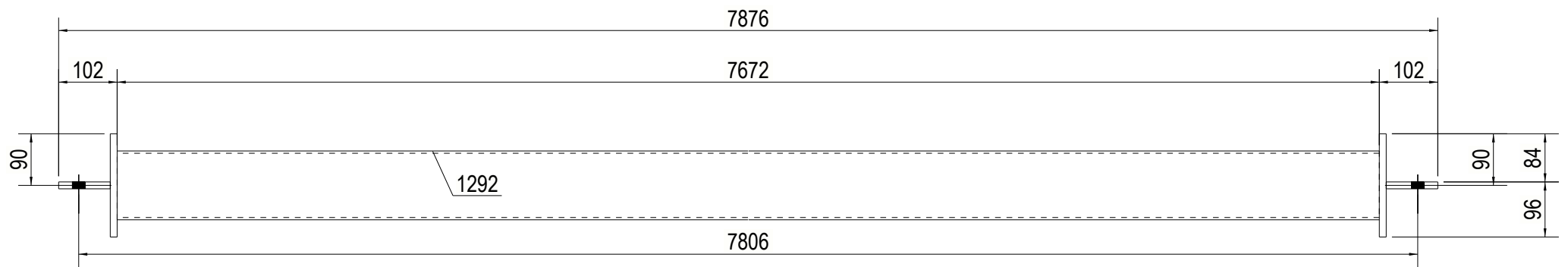
FRONT VIEW
